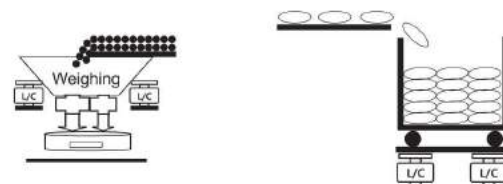
Auto Packer
