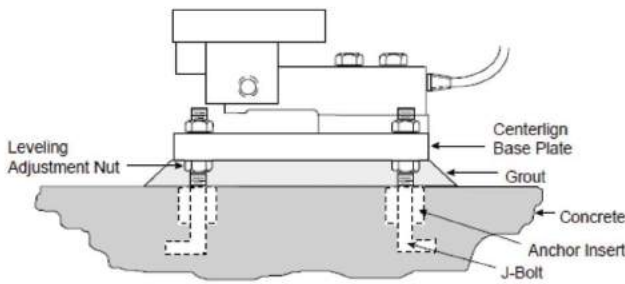
Base Plate Bolted to Unlevel Concrete Floor
