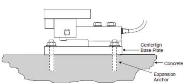
Base Plate Bolted to Level Concrete Floor
