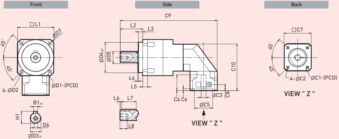
Drawing of Planetary Gearbo
